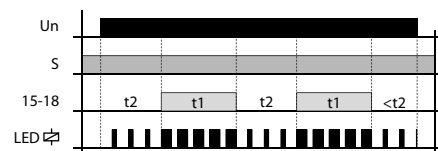
Asymmetric FLASHER - OFF first (jumper S-A1)
